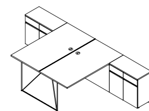
1600x3200, H=740
