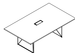
2200x1300, H=740
